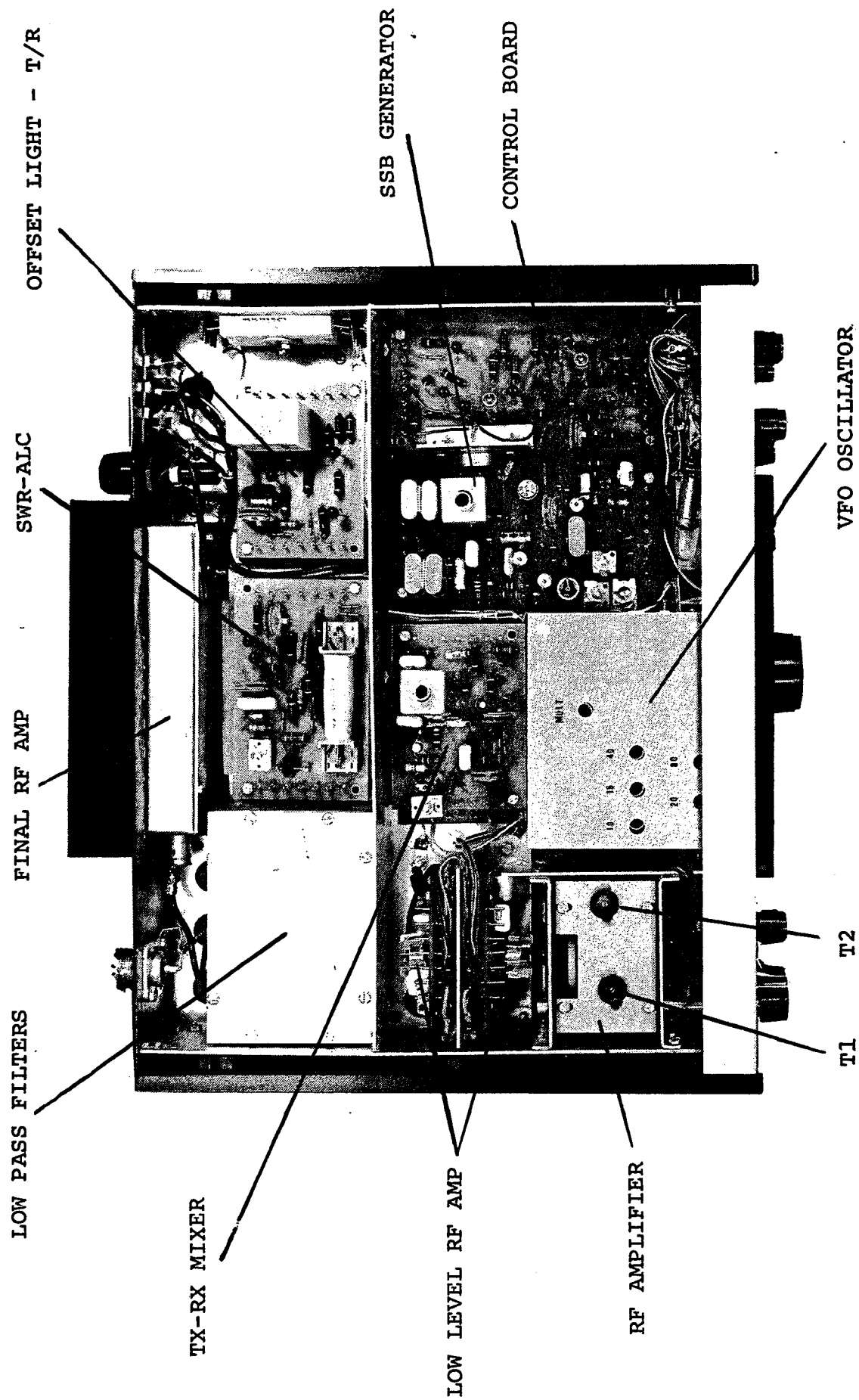
FIGURE 1 - TOP VIEW
