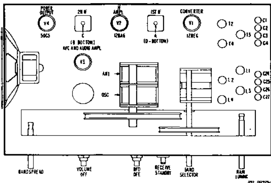
Figure 4. Chassis, Top View
