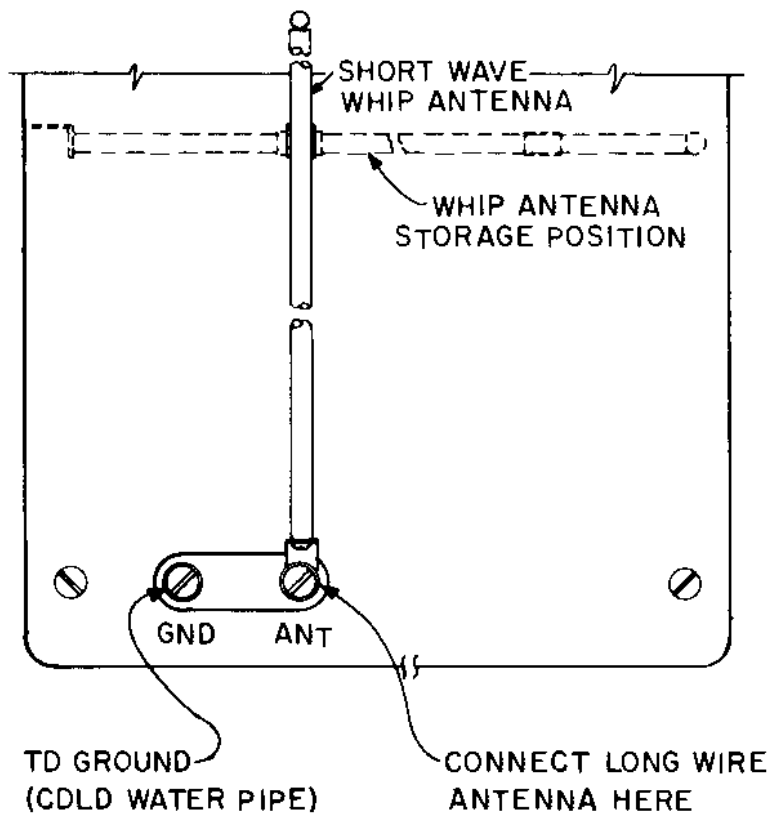
Fig. 1. Whip and Single-Wire Antenna
