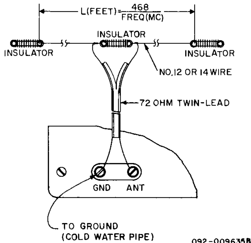
Fig. 2. Doublet Antenna
