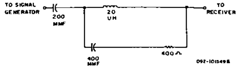
Figure 3. EIA Dummy Antenna
