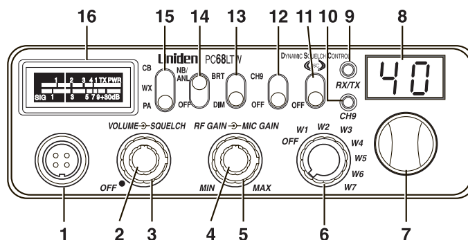
FRONT VIEW PC68LTW BACKLIGHTED PANEL
