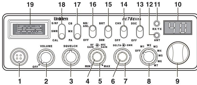
FRONT VIEW - PC78 Elite BACKLITTED PANEL
