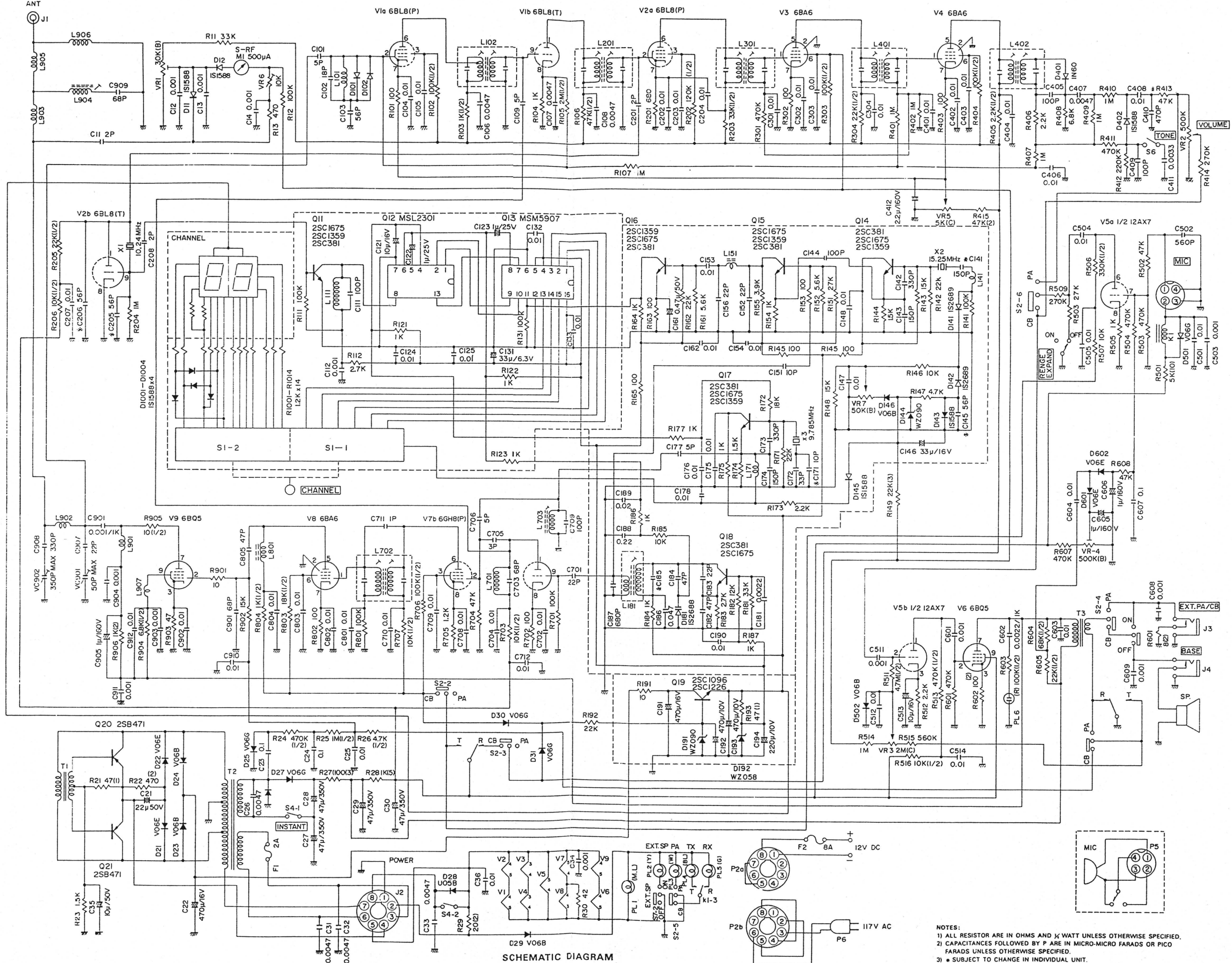
SCHMATIC DIAGRAM
