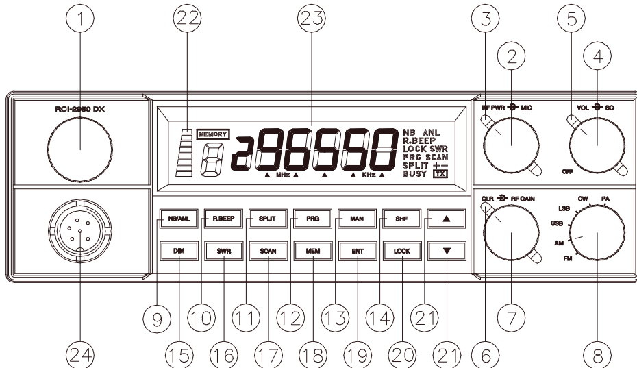
Figure 3-1 Front Panel
