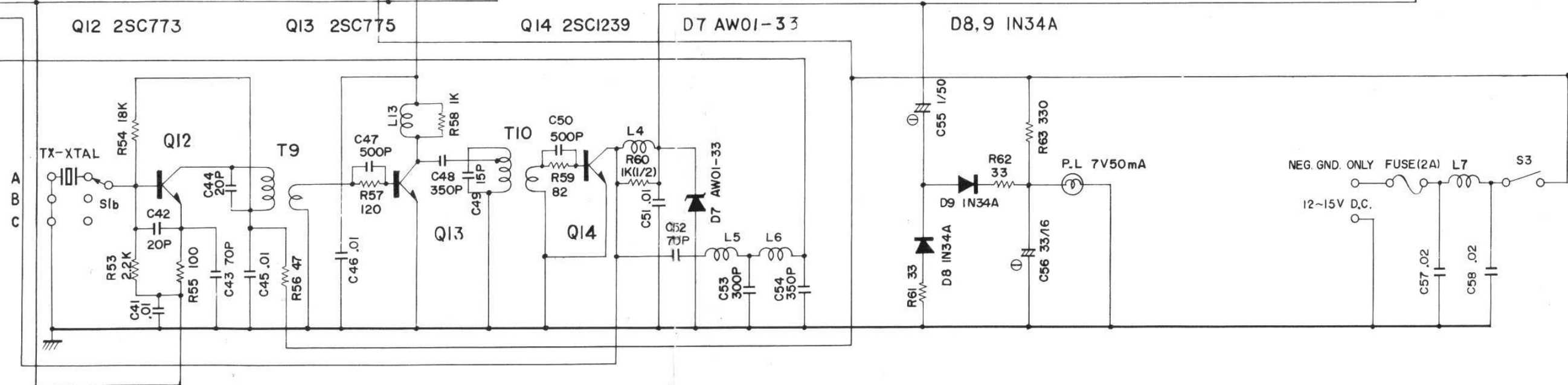
SCHMATIC DIAGRAM
